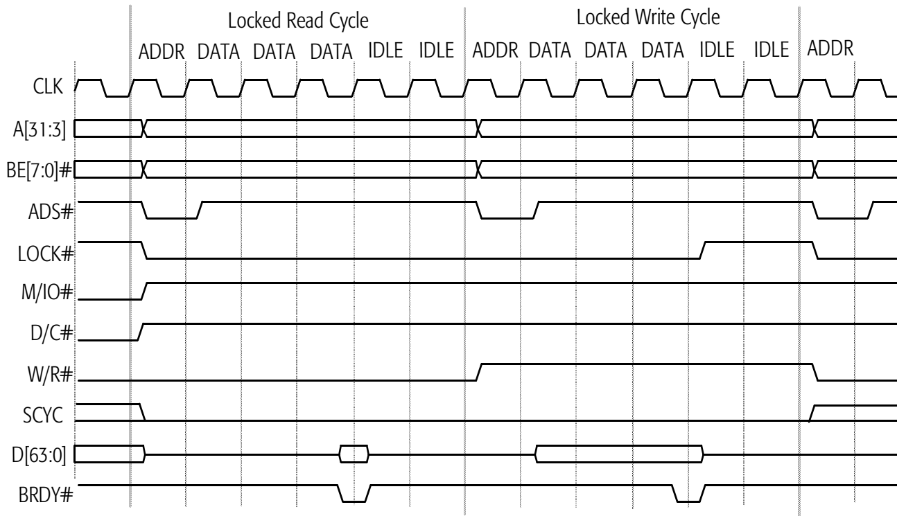
Figure 64. Basic Locked Operation
