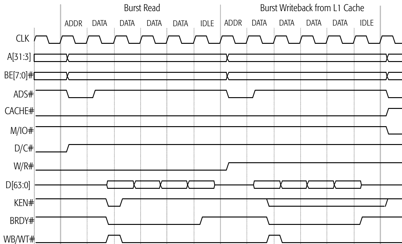
Figure 53. Burst Writeback due to Cache-Line Replacement
