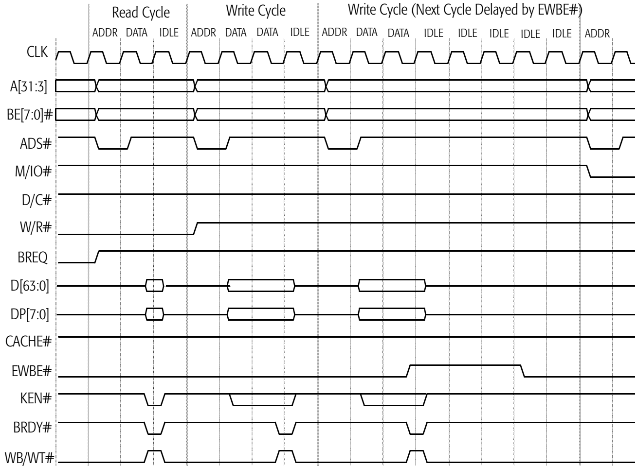
Figure 50. Non-Pipelined Single-Transfer Memory Read/Write and Write Delayed by EWBE#
