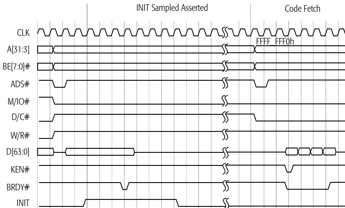
Figure 71. INIT-Initiated Transition from Protected Mode to Real Mode
