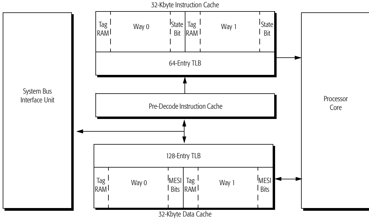
Figure 72. Cache Organization
