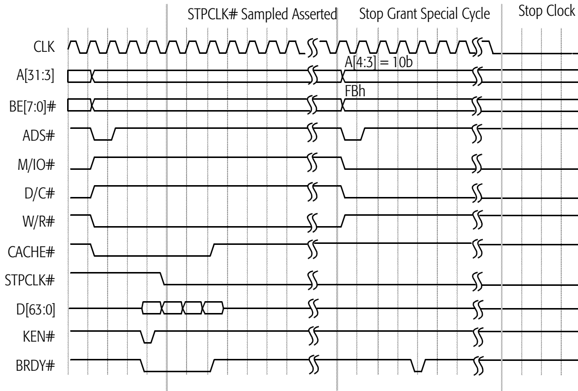
Figure 69. Stop Grant and Stop Clock Modes, Part 1
