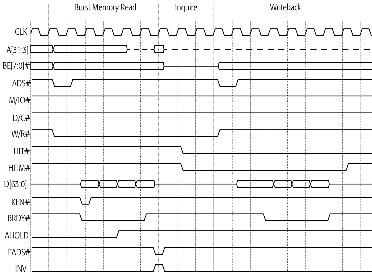
Figure 61. AHOLD-Initiated Inquire Hit to Modified Line
