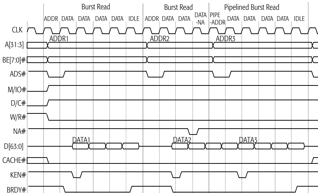
Figure 52. Burst Reads and Pipelined Burst Reads
