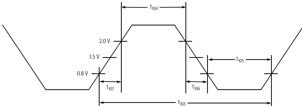
Figure 93. TCK Waveform
