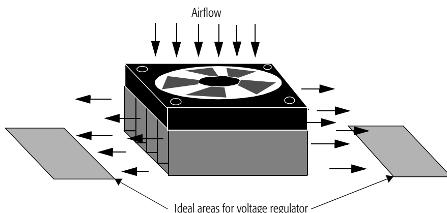
Figure 101. Airflow for a Heatsink with Fan
