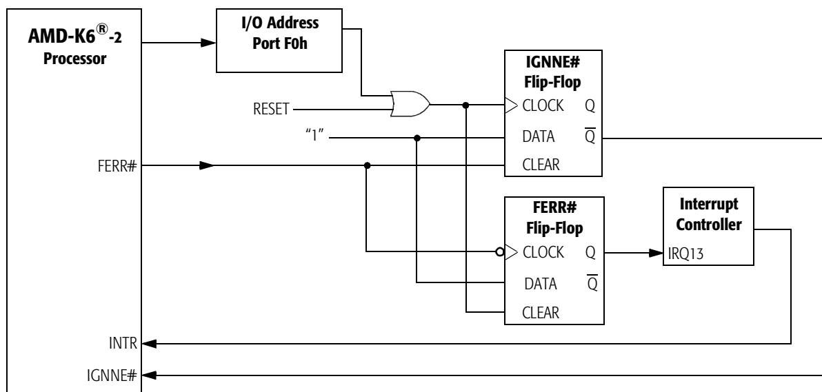
Figure 76. External Logic for Supporting Floating-Point Exceptions
