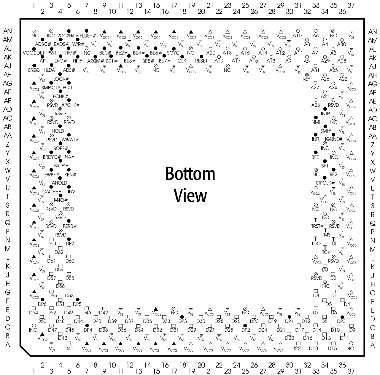
Figure 105. AMD-K6 ® -2 Processor Pin-Side View
