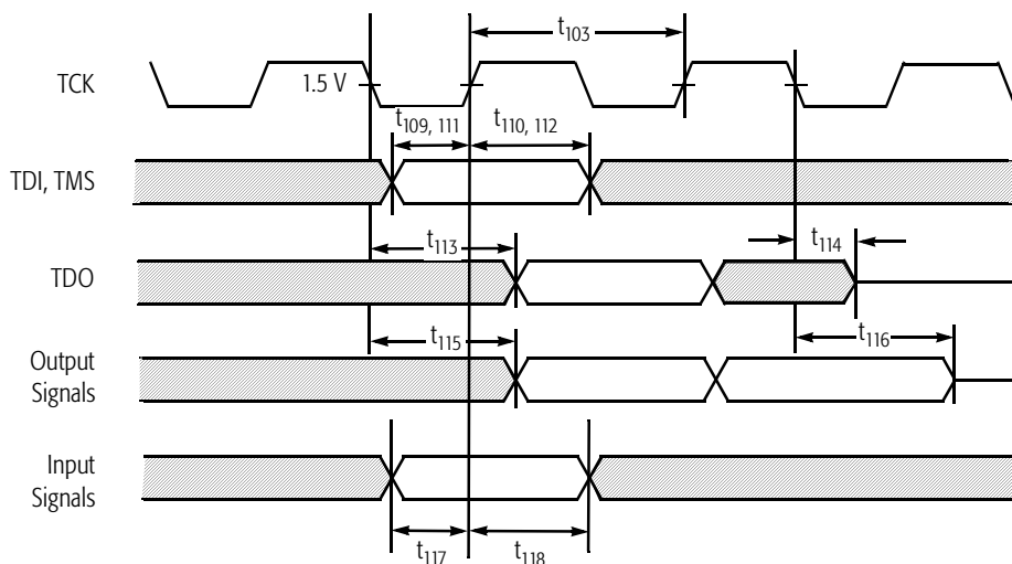
Figure 95. Test Signal Timing Diagram
