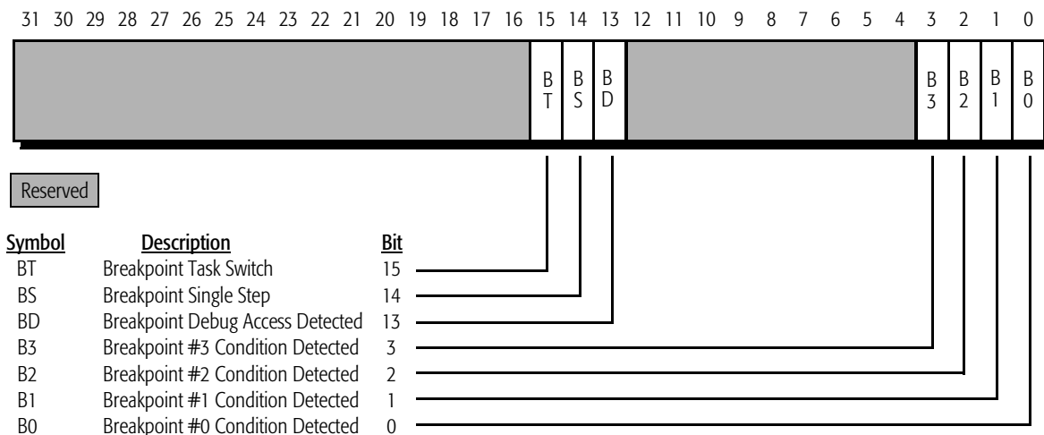
Figure 80. Debug Register DR6
