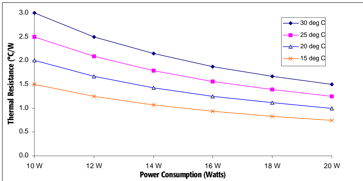
Figure 97. Power Consumption vs. Thermal Resistance
