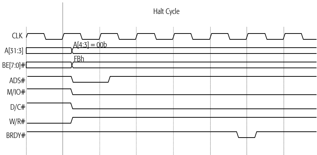
Figure 67. Basic Special Bus Cycle (Halt Cycle)
