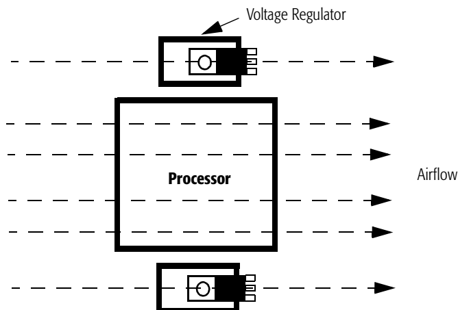
Figure 100. Voltage Regulator Placement
