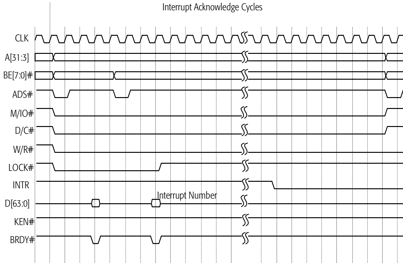
Figure 66. Interrupt Acknowledge Operation
