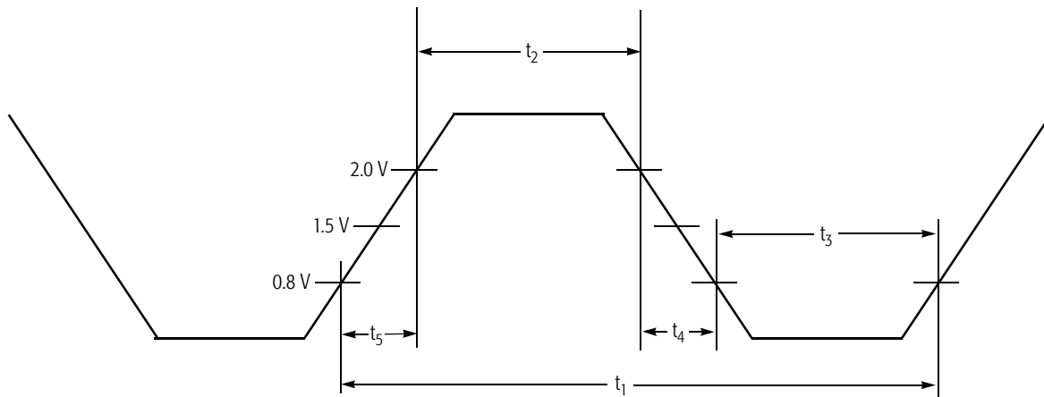
Figure 87. CLK Waveform
