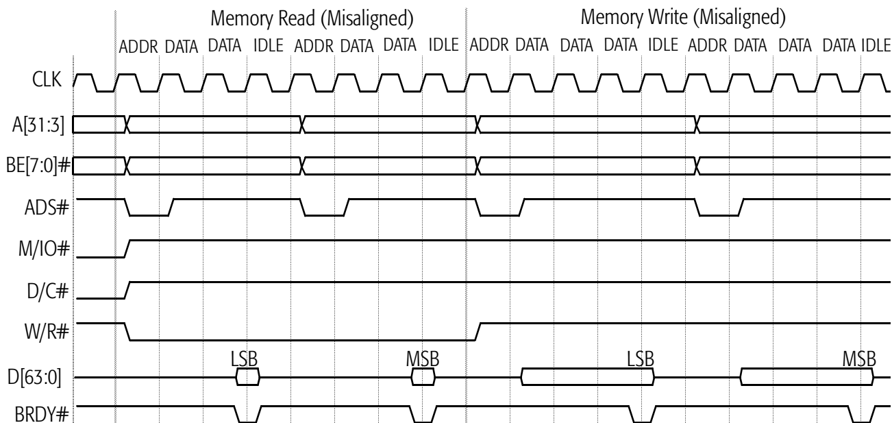
Figure 51. Misaligned Single-Transfer Memory Read and Write
