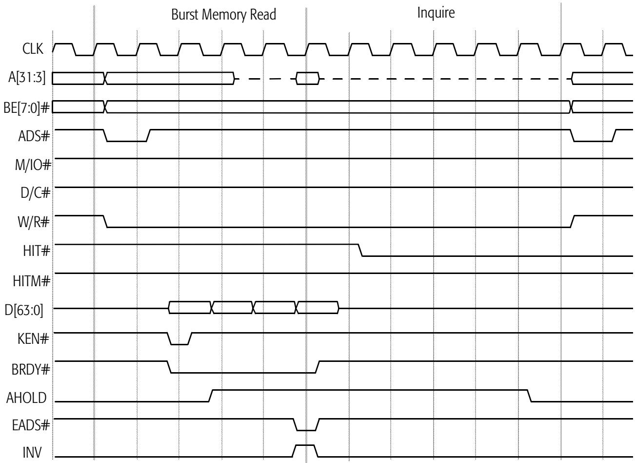
Figure 60. AHOLD-Initiated Inquire Hit to Shared or Exclusive Line
