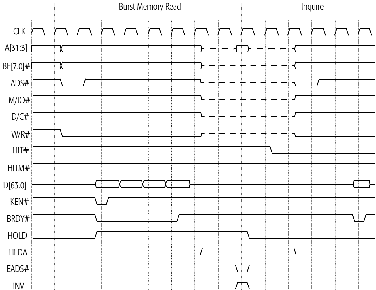
Figure 57. HOLD-Initiated Inquire Hit to Shared or Exclusive Line
