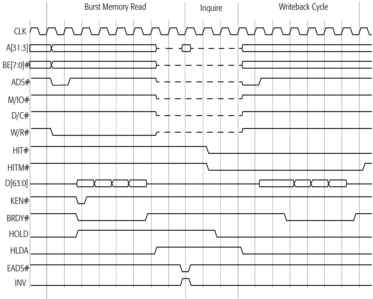
Figure 58. HOLD-Initiated Inquire Hit to Modified Line
