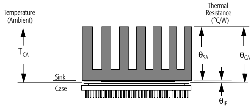
Figure 96. Thermal Model
