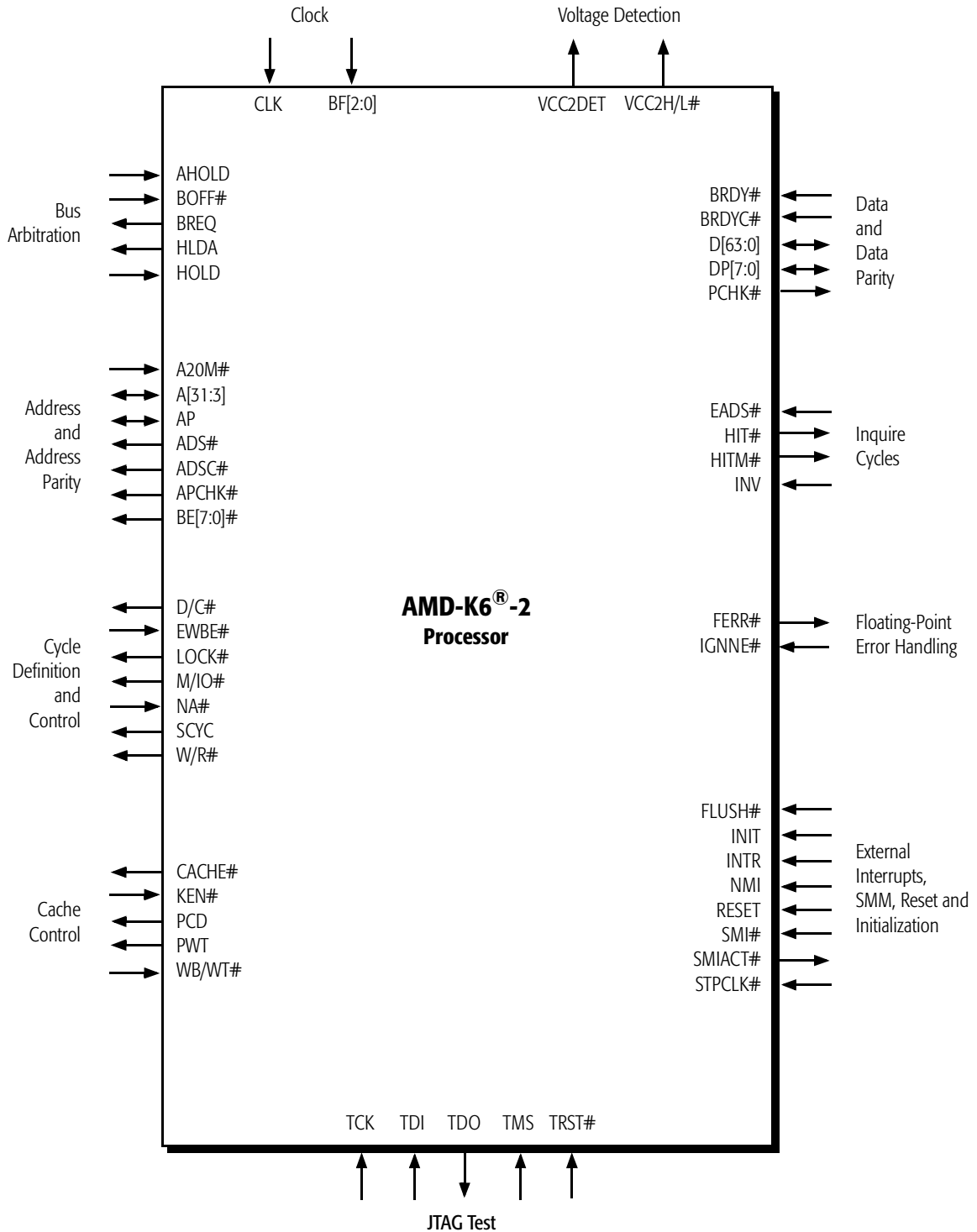
Figure 47. Logic Symbol Diagram
