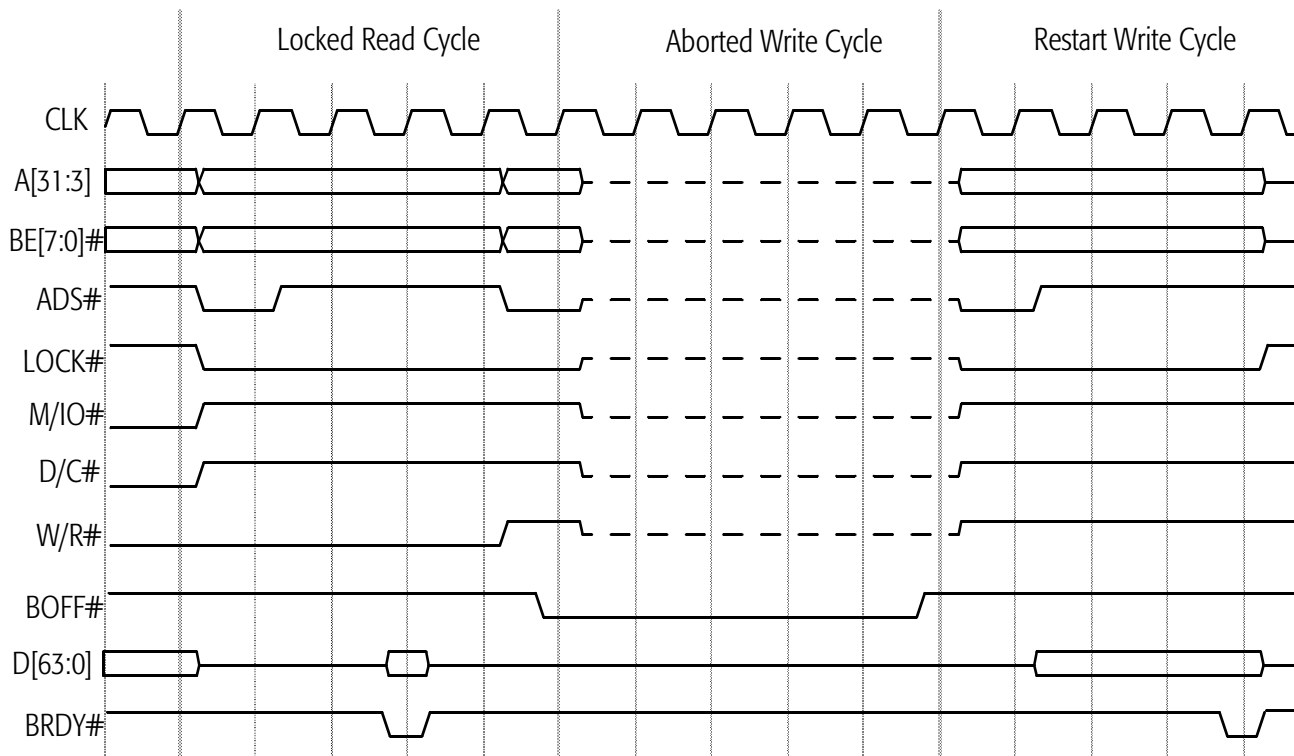
Figure 65. Locked Operation with BOFF# Intervention
