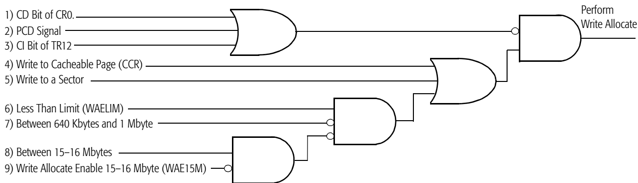
Figure 75. Write Allocate Logic Mechanisms and Conditions
