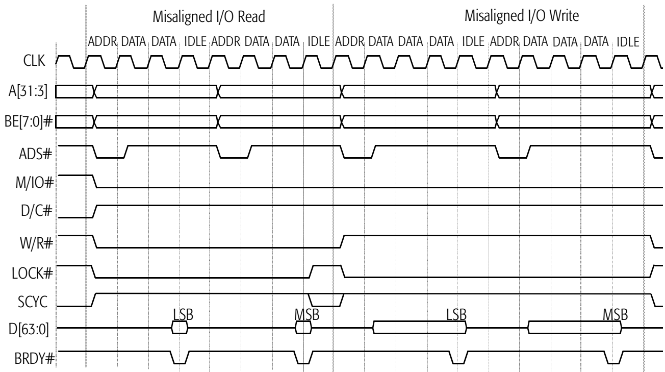
Figure 55. Misaligned I/O Transfer
