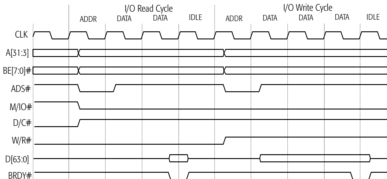
Figure 54. Basic I/O Read and Write
