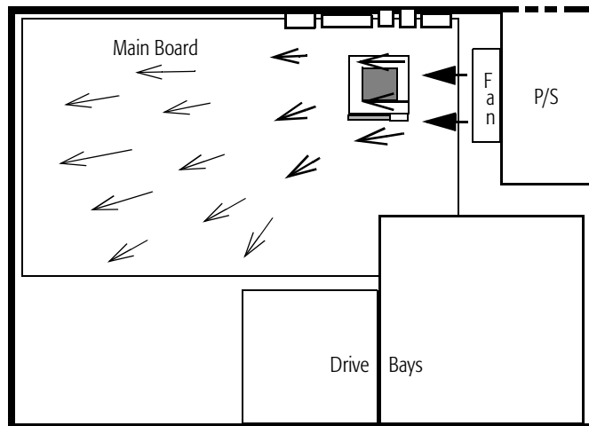
Figure 103. Airflow Path in an ATX Form-Factor System
