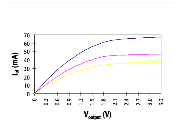
Figure 85. K6STD Pulldown V/I Curves
