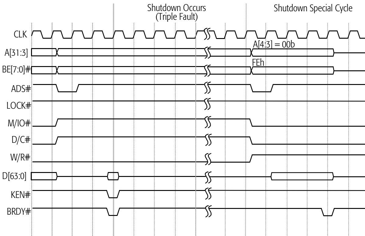
Figure 68. Shutdown Cycle
