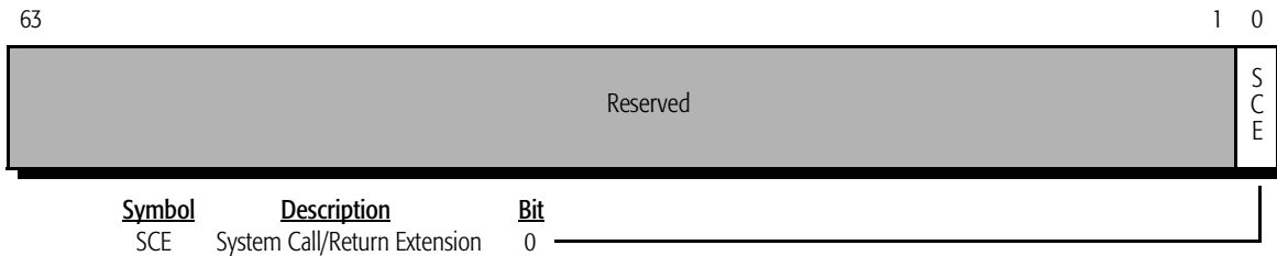
Figure 34. Extended Feature Enable Register (EFER)
