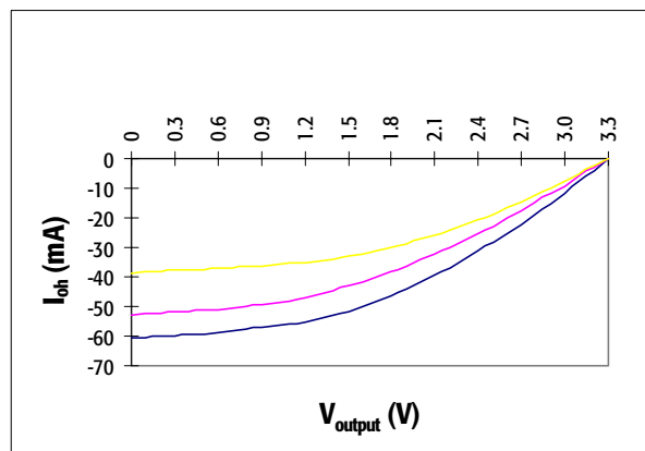
Figure 86. K6STD Pullup V/I Curves
