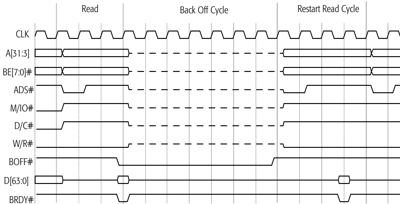
Figure 63. BOFF# Timing
